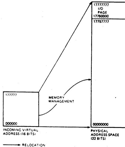
Figure 4-13 22-Bit Mapping
