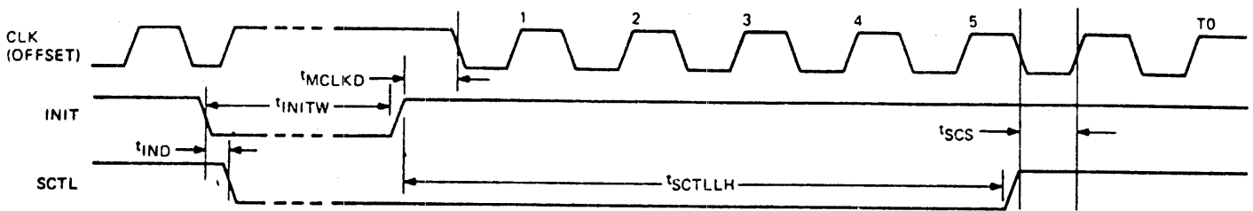
Figure 8-1 Initialization
