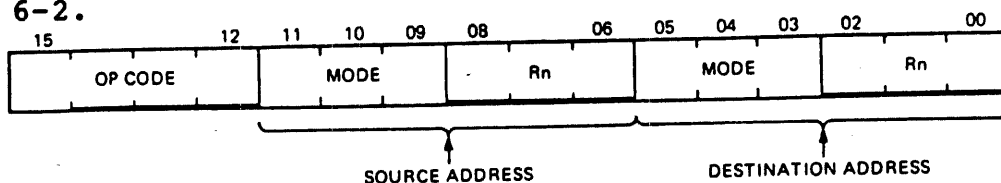
Figure 6-2 Double-Operand Addressing
