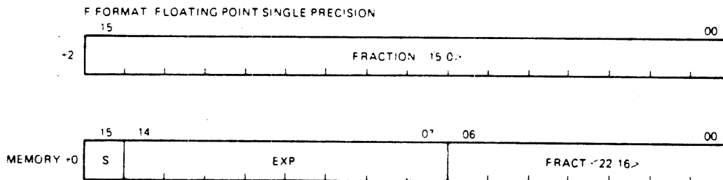
Figure 7-1 Single-Precision Format
