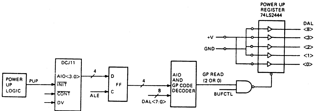
Figure 8-4 Power-Up Circuit
