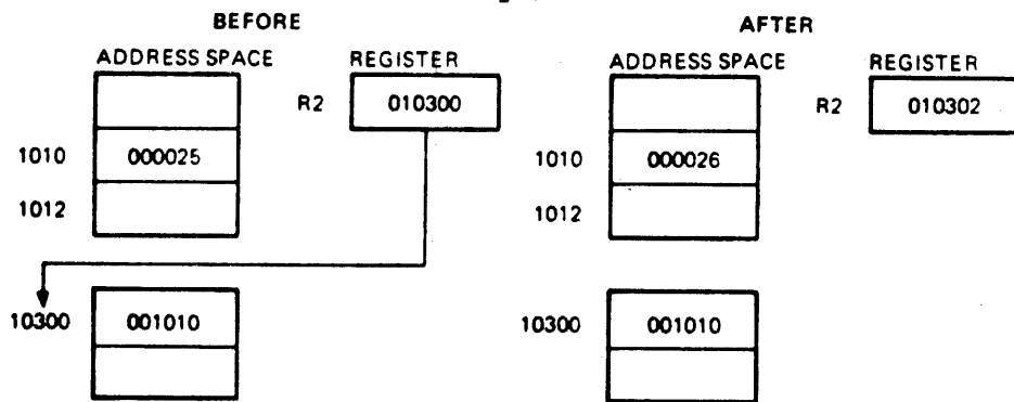
Figure 6-24 INC @(R2)+ Increment
