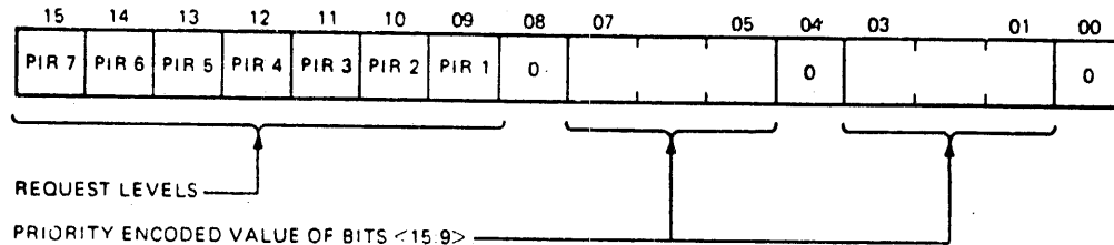
Figure 1-4 PIRQ Register
