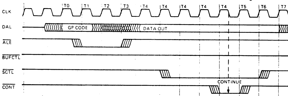
Figure 3-7 General-Purpose Write Cycle
