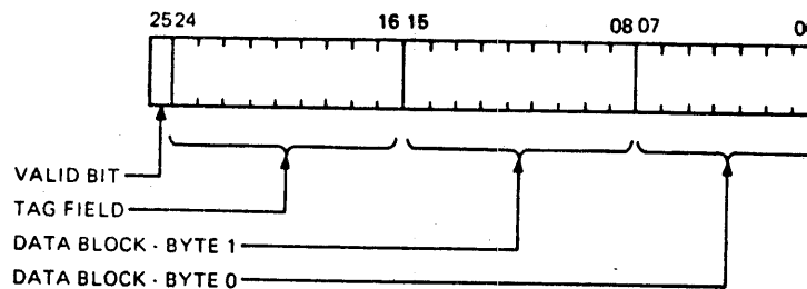
Figure 5-4 Cache Entry
