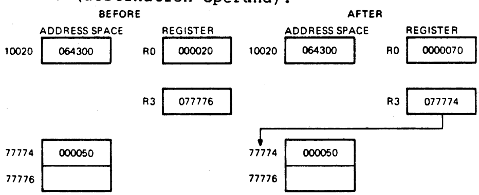
Figure 6-15 ADD -(R3),R0 Add
