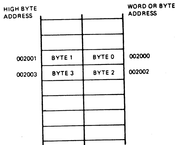
Figure 6-46 Byte Instructions
