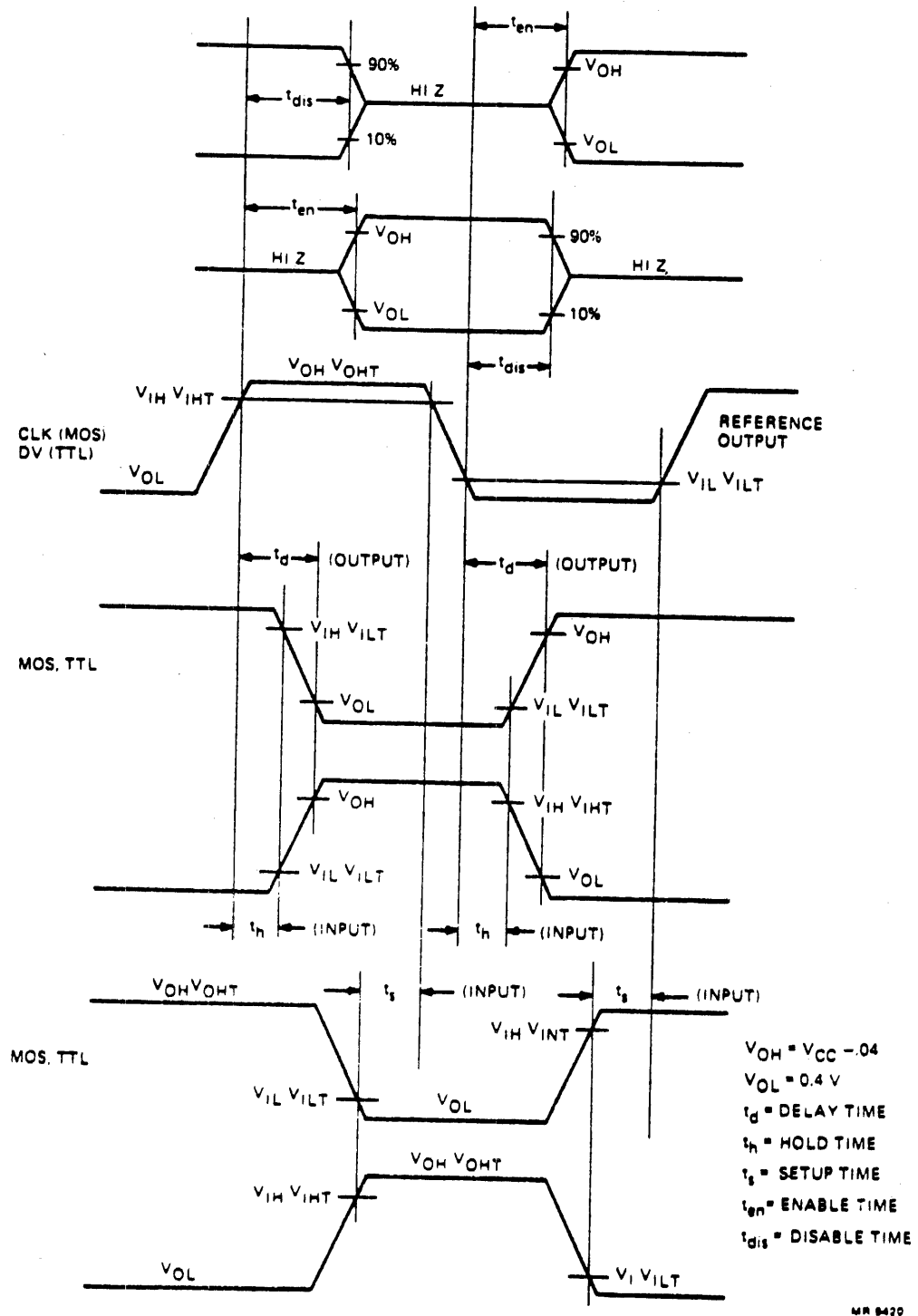
Figure A-1 Voltage Waveforms
