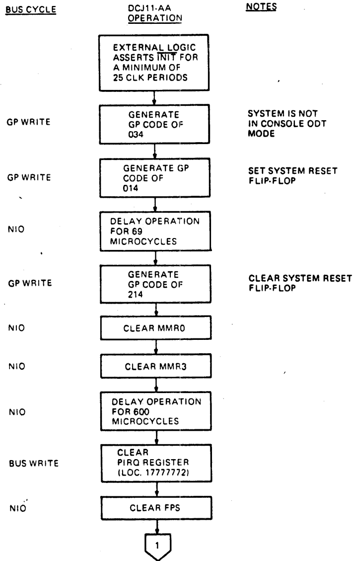
Figure 8-2 Initialization Sequence
