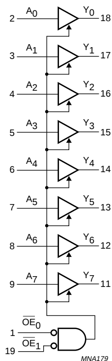
Fig.2 Logic symbol.
